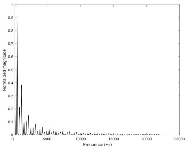
Figure 4: Normalized LTAS for the reed source signal simulated using physics model.
