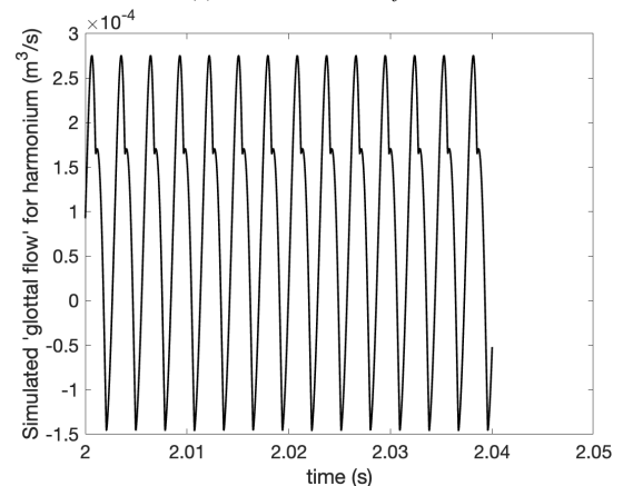
(b) Simulated reed airflow.
