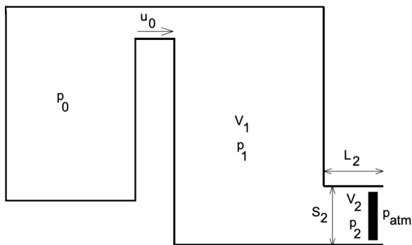
Figure 2: Configuration of the Physical model.
