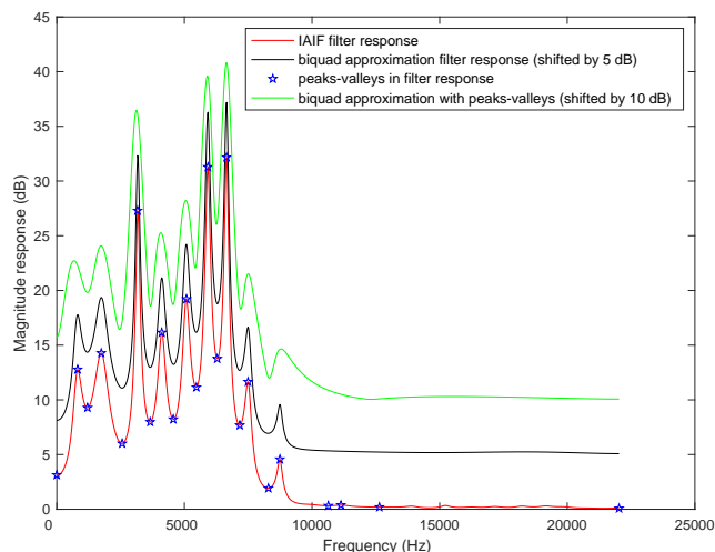
Figure 5: Frequency response of estimated and approximated wooden enclosure filters for a concert quality harmonium.
