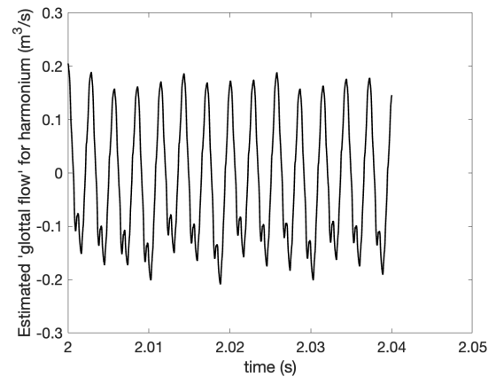
(a) Estimated reed airflow.
