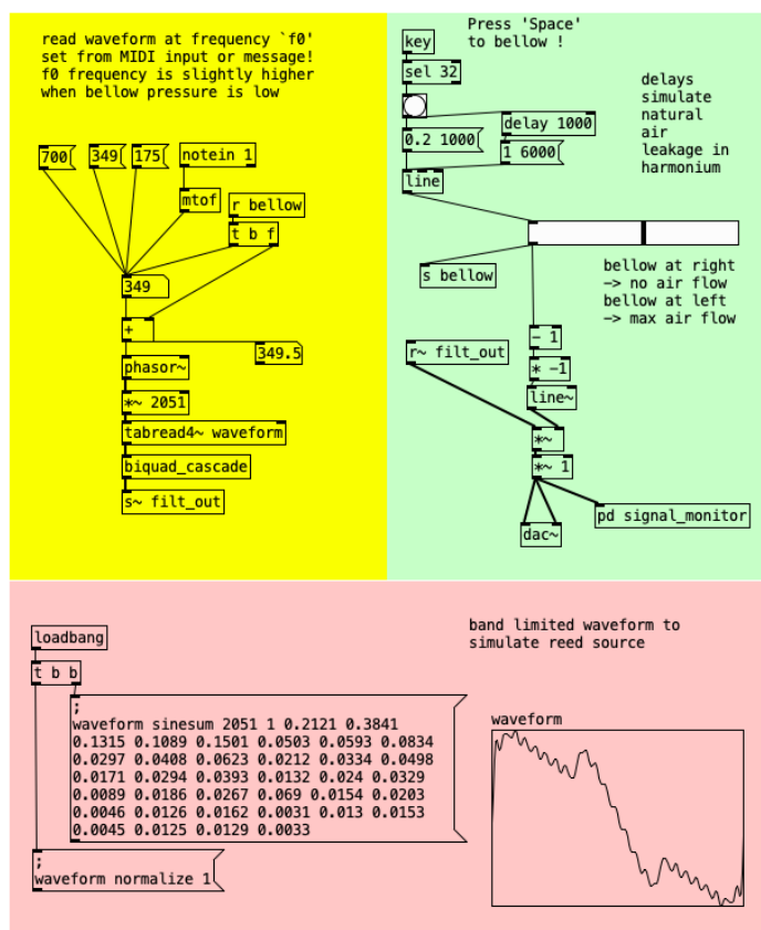
Figure 6: Pure Data patch to implement the signal model.
