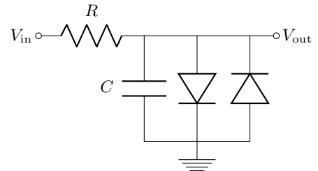
Figure 4: Diagram of the diode clipper circuit.
