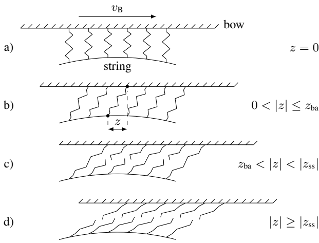
Figure 1: Microscopic displacements of the bristles between the bow and the string. The bow moves right with a velocity of v_B . a) The initial state is where the average bristle displacement z = 0 . b) The bow has moved right relative to the string. The purely elastic, or presliding regime is entered (stick). c) After the break-away displacement z_{ba} , more and more bristles start to ‘break’. This is defined as the elasto-plastic regime. d) After all bristles have ‘broken’, the steady state (slip) is reached and the purely plastic regime is entered.
