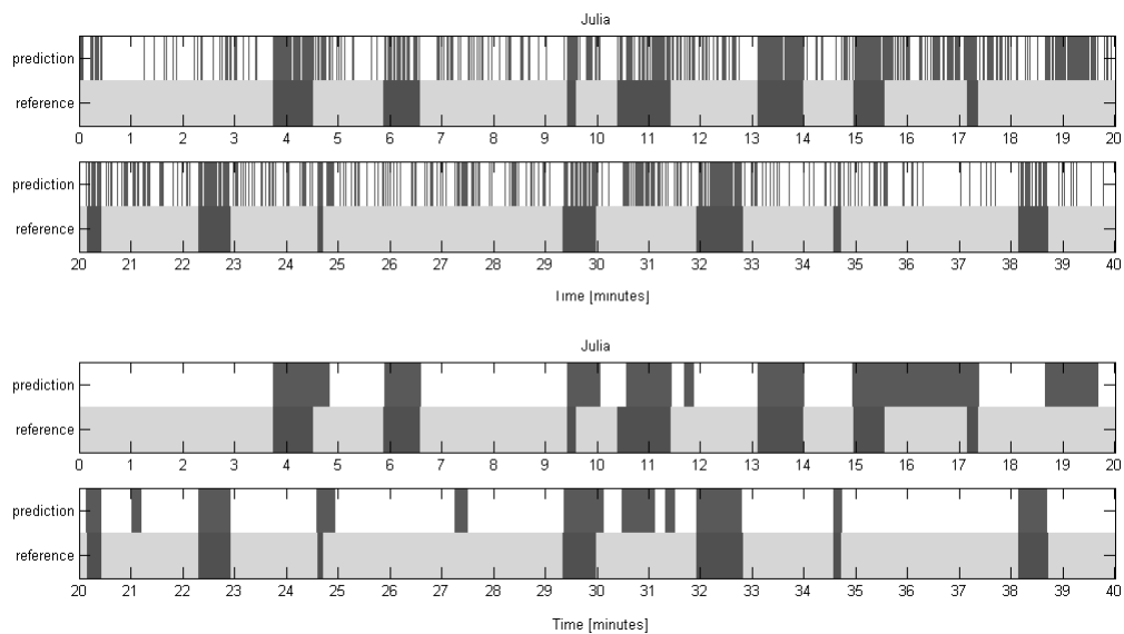
Figure 4: Visualization of the classification results for the machine learning approach of 40 minutes of the soap opera "Julia". Each line represents 20 minutes of audio and is split to compare the class prediction with the true class. The class "music" is represented by a lighter color, whereas "no_music" is in the form of dark regions. The lower subplot illustrates the results after the application of the smoothing function.
