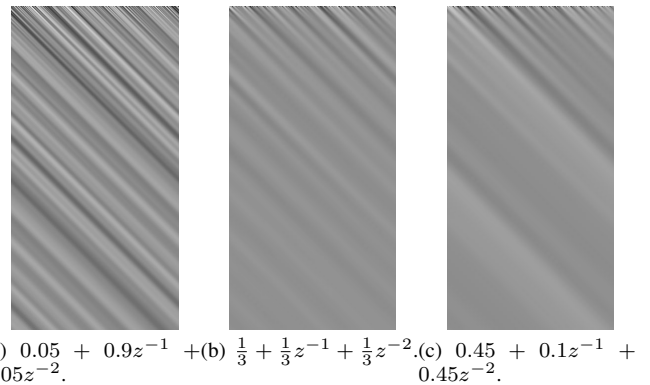
Figure 14: Rastrogams of the same Karplus-Strong model as figure 4.1, with different second-order loop filter H(z) s that introduce one sample delay.
