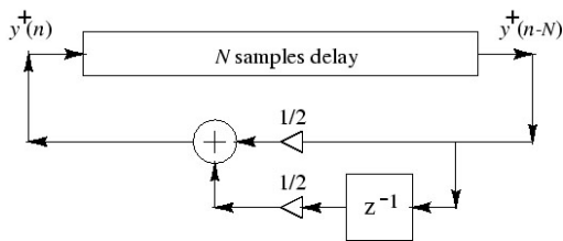
Figure 12: System diagram of Karplus-Strong algorithm, with a simple loop filter.
