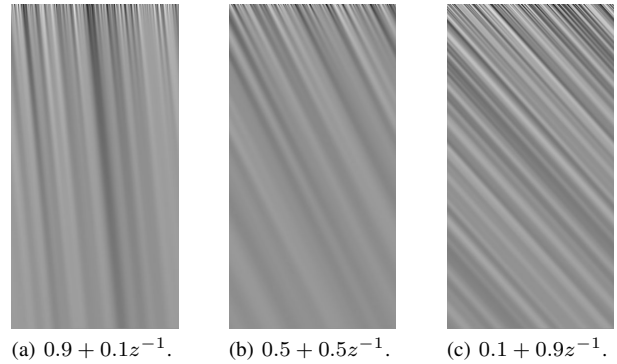
Figure 13: Rastrogams of plucked-string sounds generated from Karplus-Strong algorithm, with different loop filter H(z) s as individually specified. Delay line length N is 337, which corresponds to about 130.9 [Hz].
