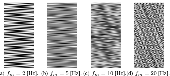
Figure 8: Rastrograms of frequency modulated sounds, y(t) = \cos[2\pi\{f_c t + I \cdot f_m \cdot \sin(2\pi f_m t)\}] , with f_c = 220.5 [Hz], I = 1 , but different f_m values (as specified).
