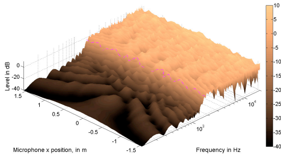
Figure 4: Frequency responses of the aliased field H_{\Psi}^{al} , source 10, regularly spaced array.
