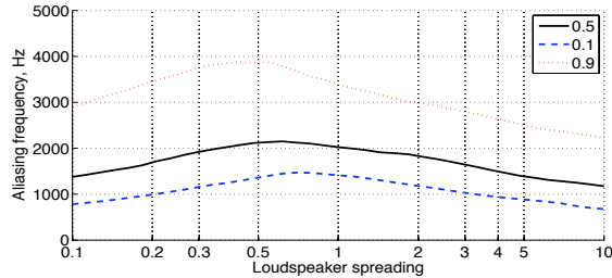
Figure 8: Quantiles of aliasing frequency, logarithmically spaced arrays, all microphone positions, loudspeaker spreading coefficient dependency, all sources.
