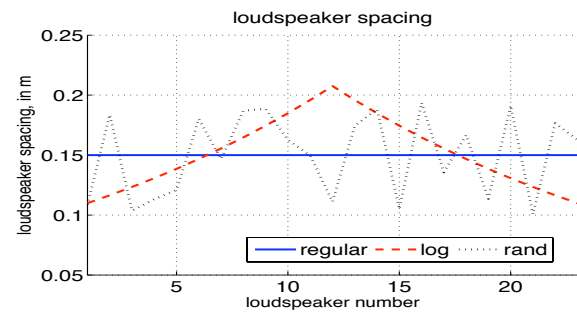
Figure 2: loudspeaker spacing for the three array type.
