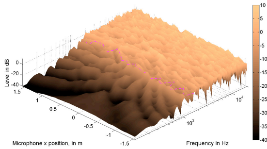
Figure 6: Frequency responses of the aliased field H_{\Psi}^{al} , source 10, randomly spaced array.
