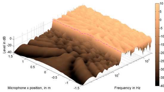
Figure 5: Frequency responses of the aliased field H_{\Psi}^{al} , source 10, logarithmically spaced array.
