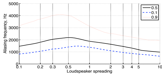
Figure 9: Quantiles of aliasing frequency, logarithmically spaced arrays, all microphone positions, spreading coefficient dependency, non-focused sources only.
