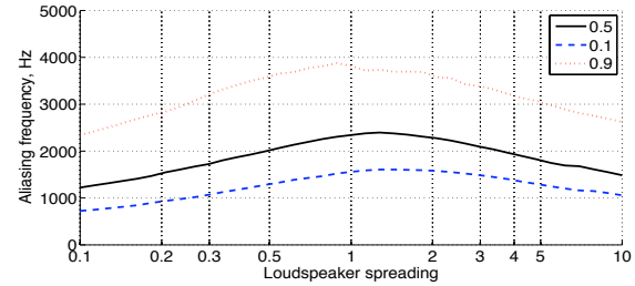
Figure 10: Quantiles of aliasing frequency, logarithmically spaced arrays, all microphone positions, spreading coefficient dependency, focused sources only
