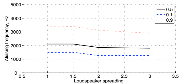
Figure 7: Quantiles of aliasing frequency, randomly spaced arrays, all sources and microphone positions, spreading coefficient dependency.
