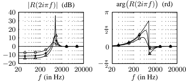
Figure 10: Bode diagrams of R for r = 0 (-), r = \frac{1}{3} (o), r = \frac{2}{3} (*) and r = 1 ( \Delta ).
