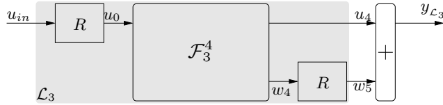
Figure 9: Third-order structure \mathcal{L}_3 of the system \mathcal{L} .
