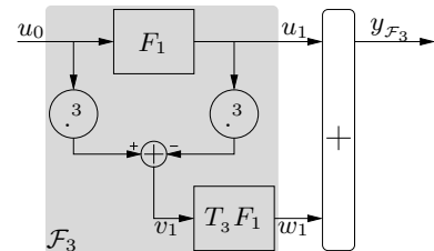
Figure 7: Third-order structure \mathcal{F}_3 of the system \mathcal{F} .
