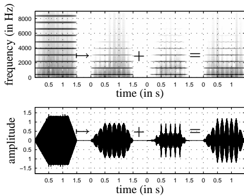
Figure 11: Spectrograms and signals of u_{in} \mapsto u_4 + u_5 = y_{L_3} .
